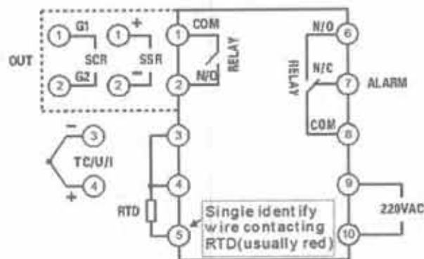
Wiring Diagram of AOB508- G series
