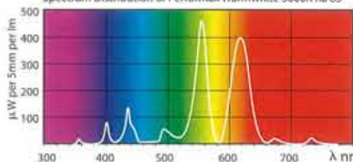
Spectrum Distribution of Performax Warmwhite 3000K Ra 85
