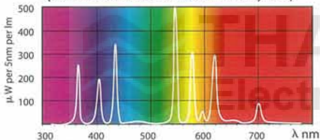
Spectrum distribution of Coated Mercury Lamp
