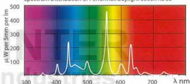
Spectrum Distribution of Performax Daylight 6500K Ra 85
