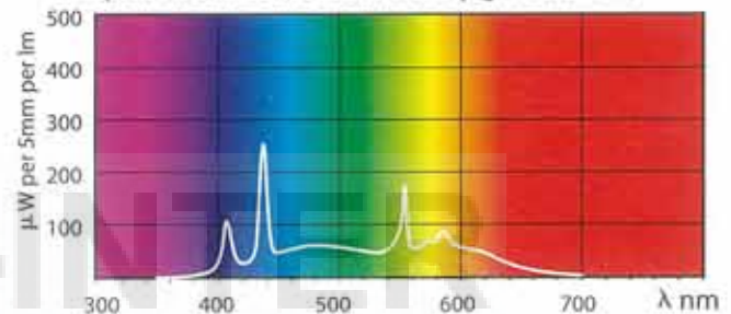
Spectrum Distribution of Standard Daylight 6200K Ra 75
