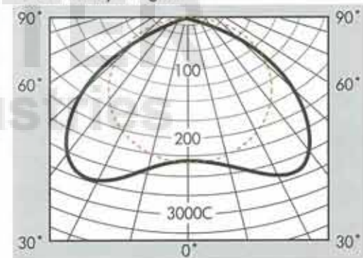
Polar Intensity Diagram
