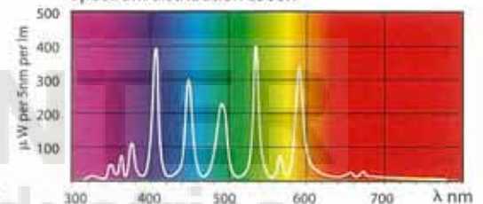
Spectrum distribution 6500K
