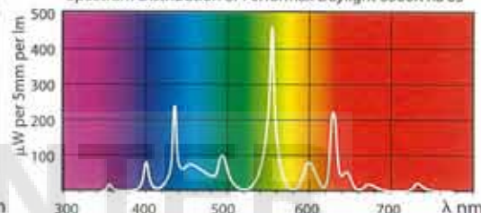
Spectrum Distribution of Performax Daylight 6500K Ra 85
