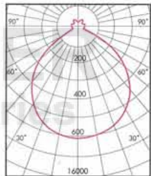
Light Intensity Diagram
