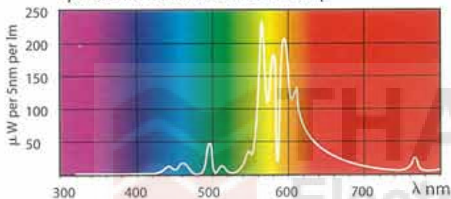
Spectrum distribution of SON Lamp
