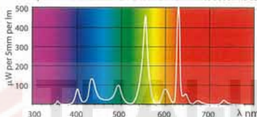
Spectrum Distribution of Performax Warmwhite 3000K Ra 85
