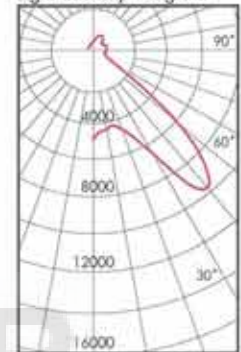
Light Intensity Diagram
